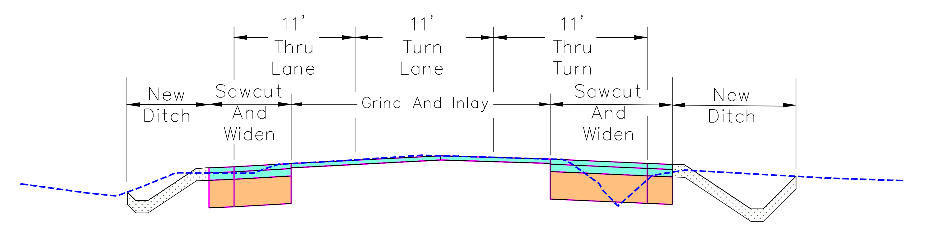
Typical Ne 179th Street Roadway Section
